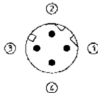
M12 4-pole Ethernet
